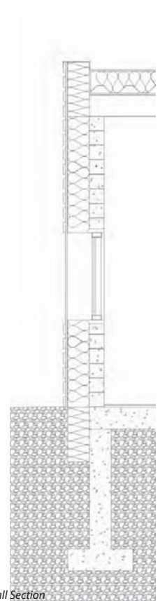
Detail Wall Section
