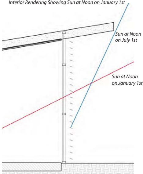
Interior Rendering Showing Sun at Noon on January 1st
