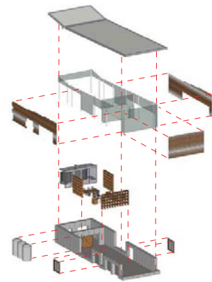
exploded axonometric
