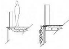
Micro Detail
